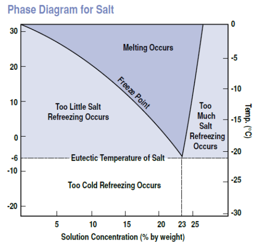
Figure 34. Phase Diagram
